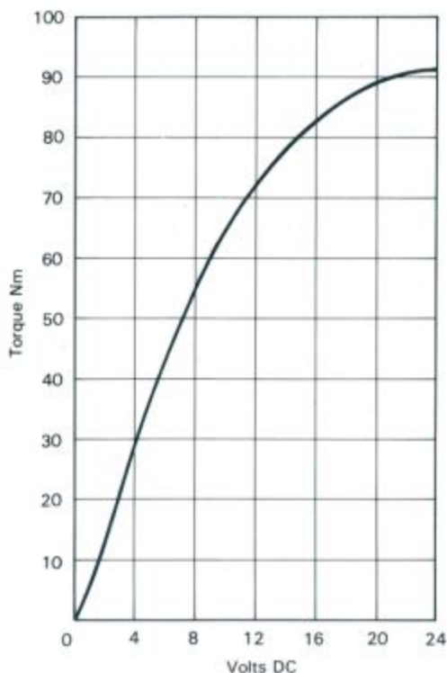
Typical Torque/voltage Characteristic PB600 Brake
