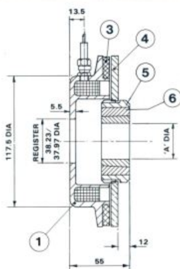
INTERNAL FLANGE MOUNTING
