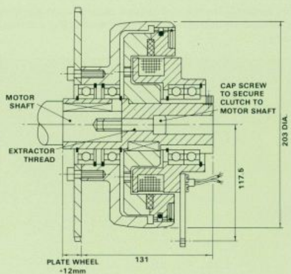
BM 800 Motor Mounting Clutch with Plate Wheel.
